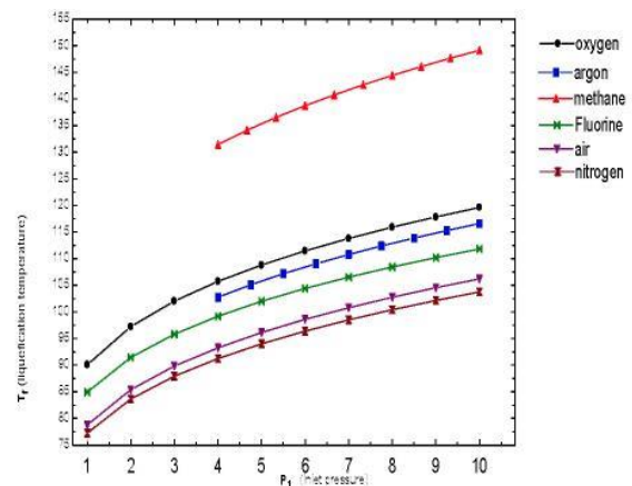
Fig 2: Variation of Liquefaction Temperature with Inlet Pressure
